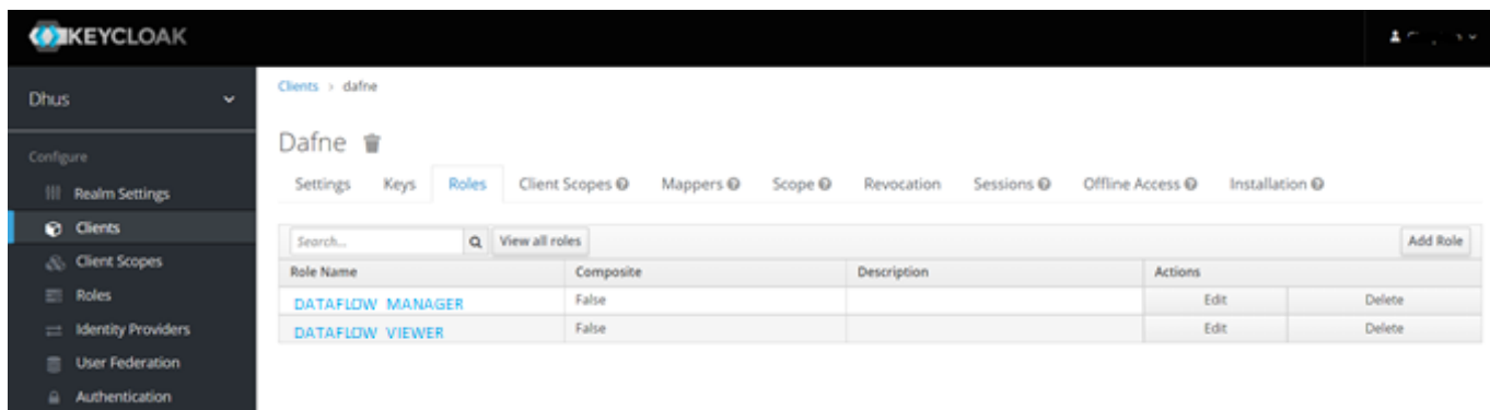
Figure 3 DAFNE Roles
