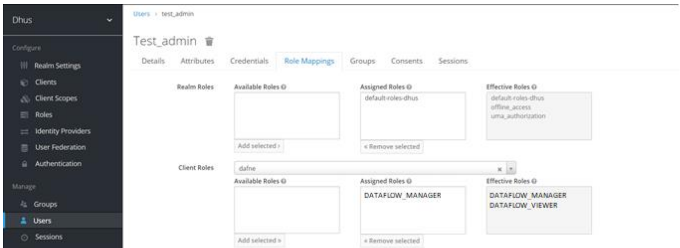
Figure 6 Assign role to DAFNE user
