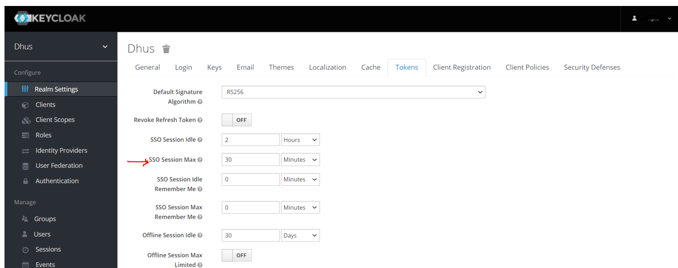
Figure 2 Token duration settings
